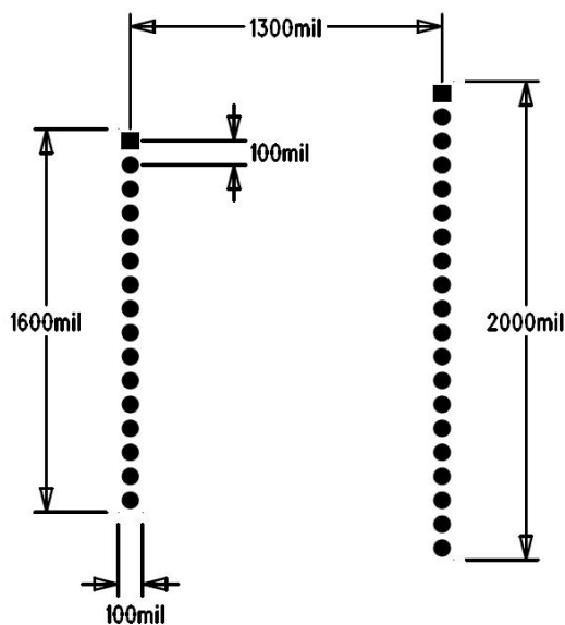
Figure 7. Board-to-board connector dimensions for the host module
