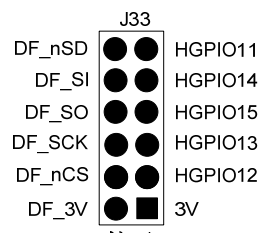
Figure 2. Jumper for DataFlash connections
