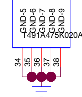
U5 FT232RQ_R 5 via grid for U5 PCB Footprint
